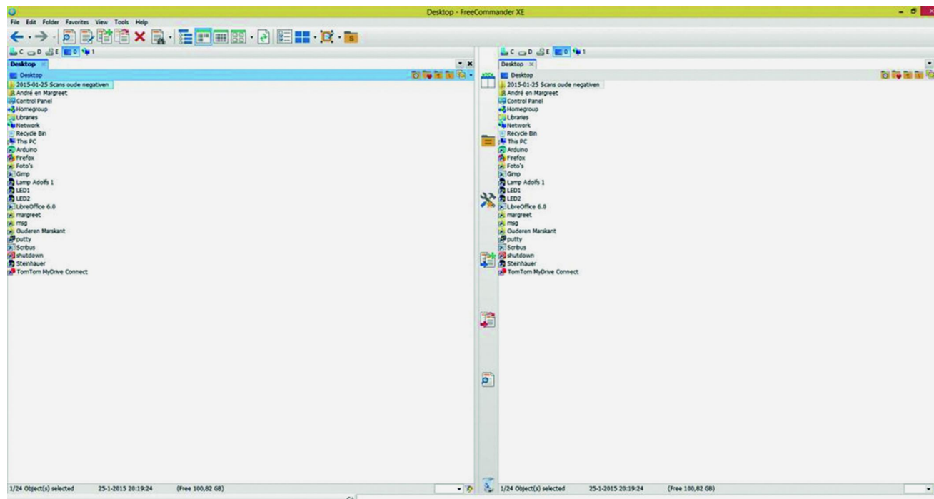
FreeCommander openingsscherm
